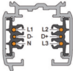
6-Line Track
